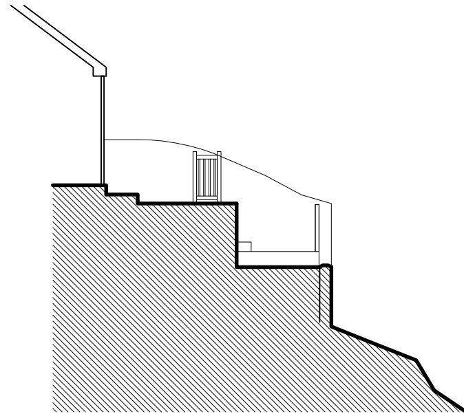
EXISTING SECTION
