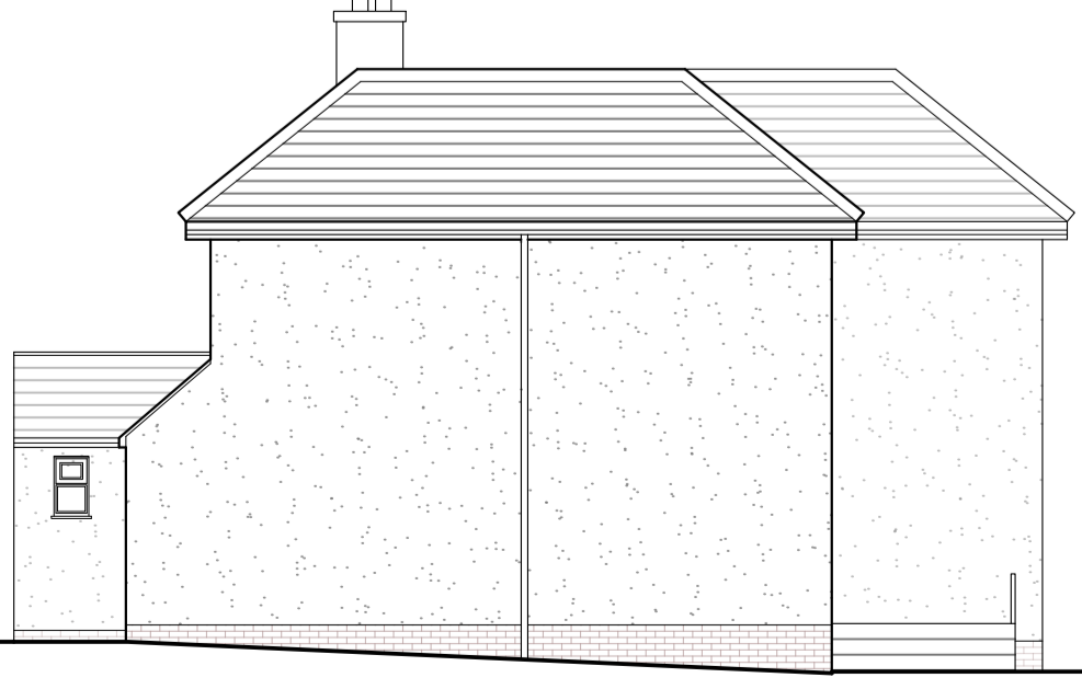
NORTH ELEVATION
