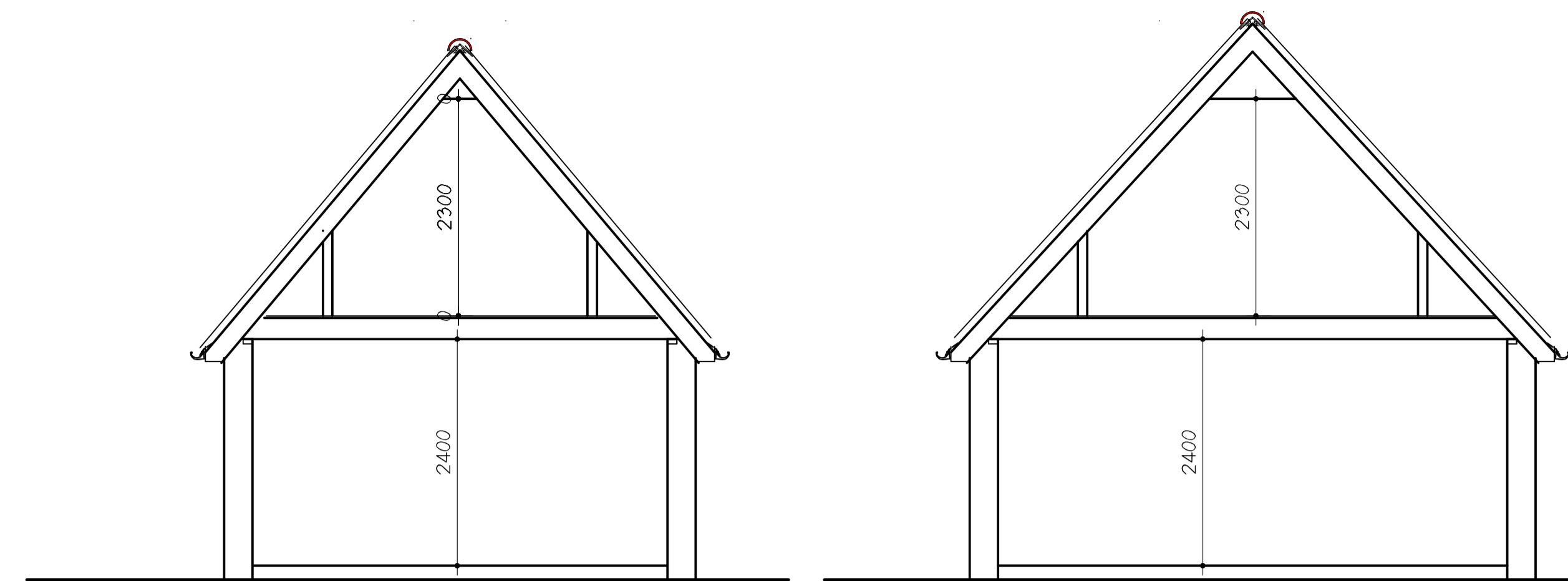
Section A - A 0 1 2 3 Section B - B Metres
