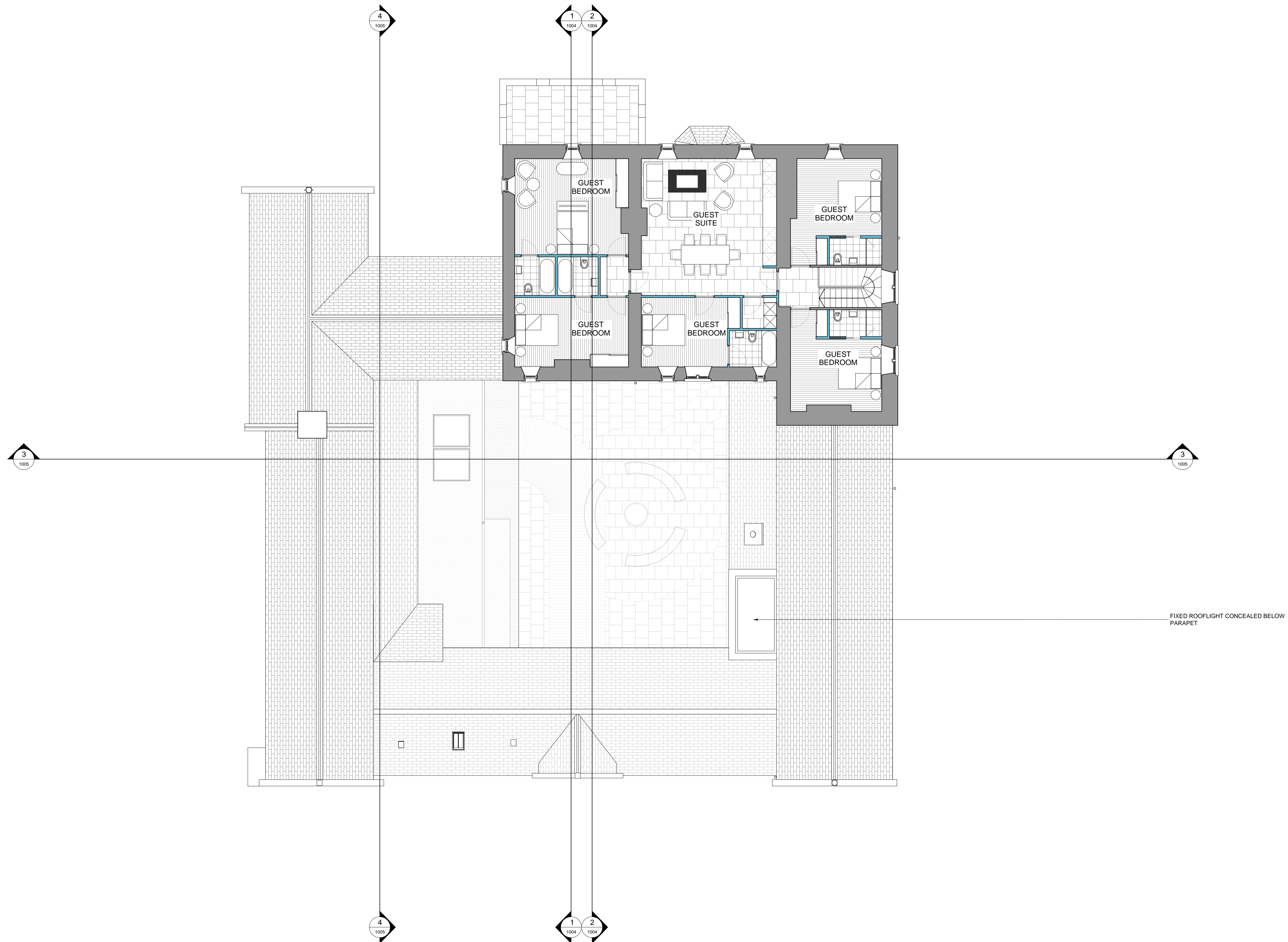
SECOND FLOOR PLAN SCALE 1:100 @ A1
