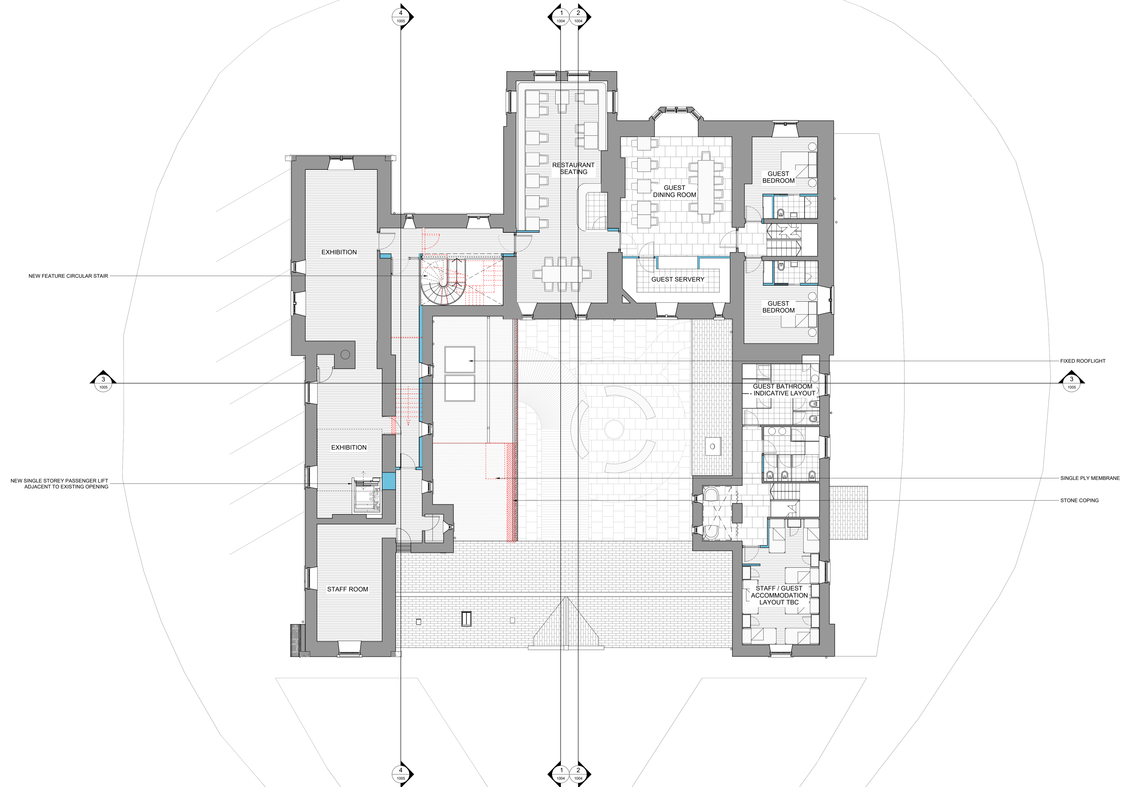
FIRST FLOOR PLAN SCALE 1:100 @ A1
