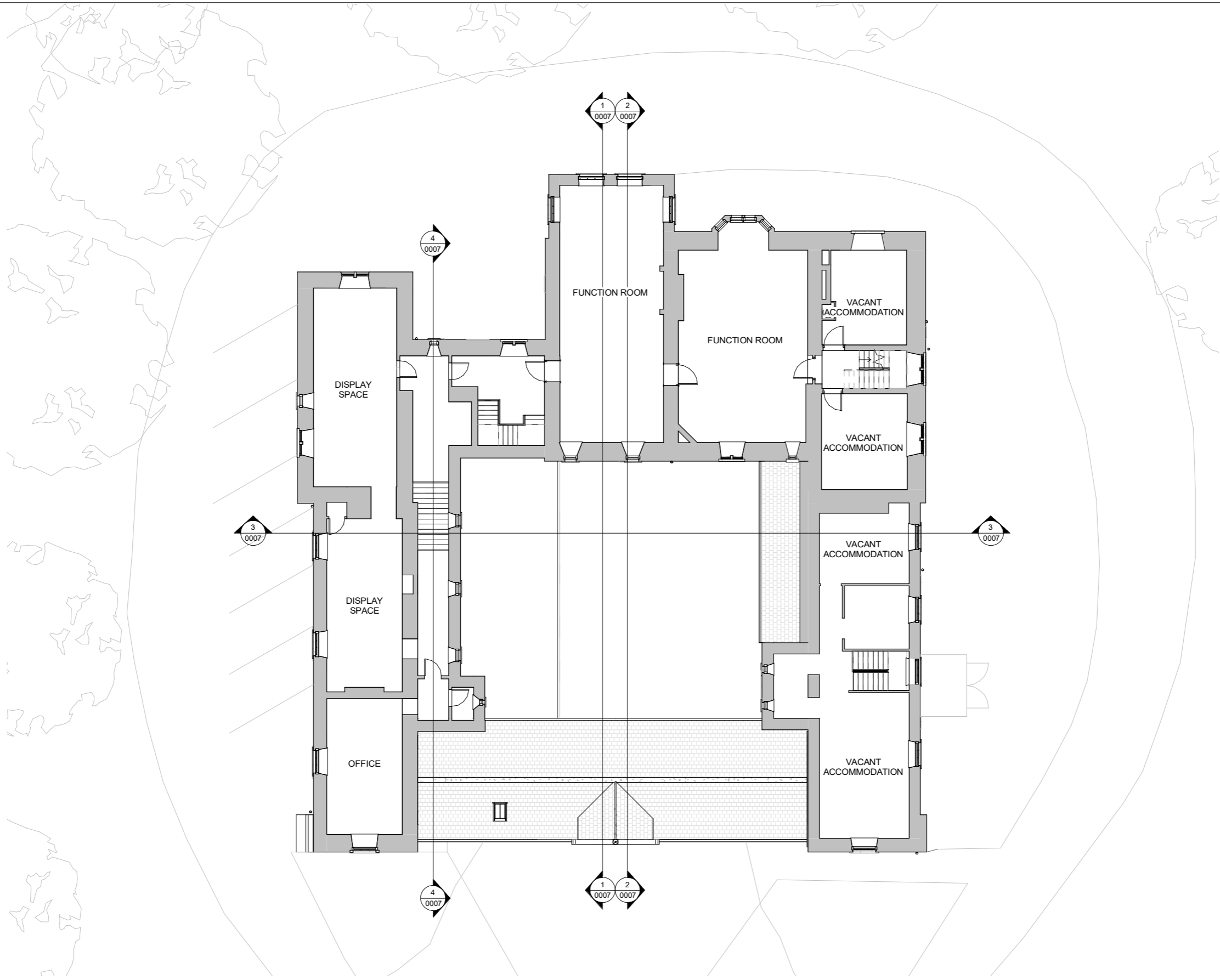
EXISTING FIRST FLOOR PLAN SCALE 1 : 200
