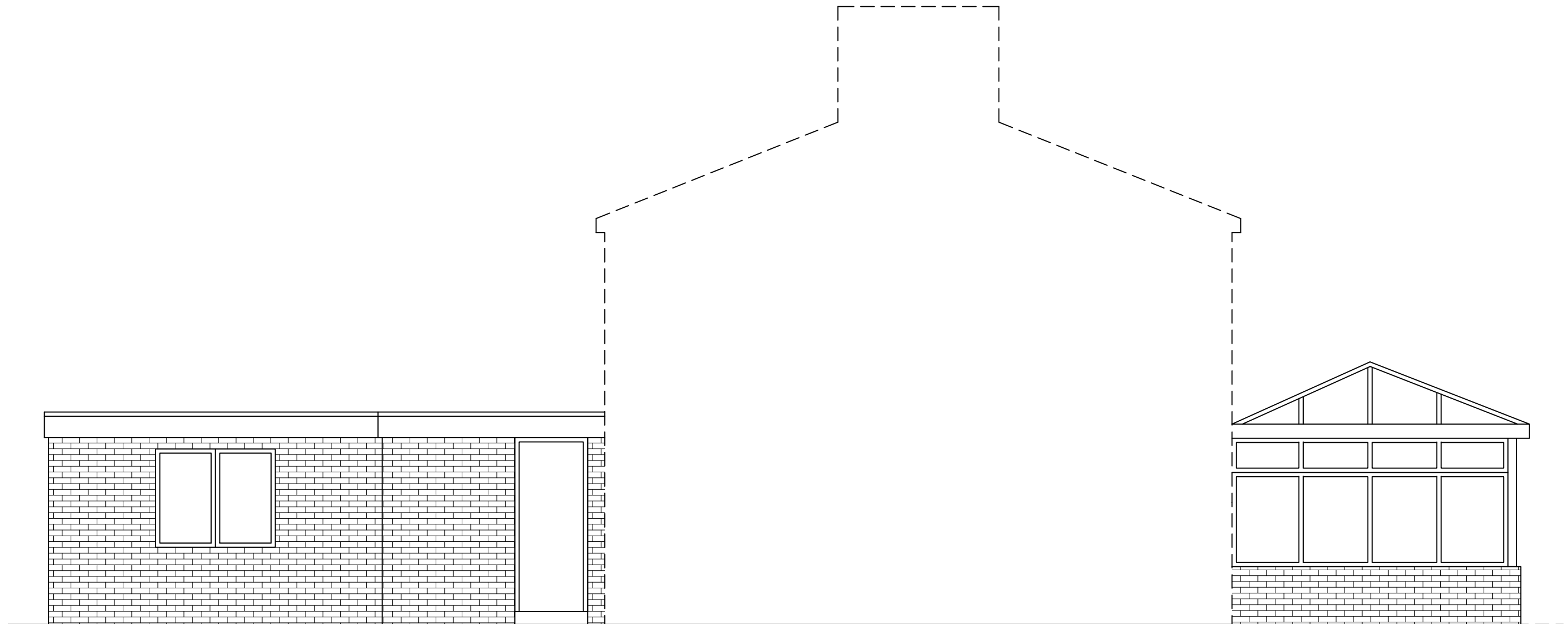
PROPOSED NORTH WEST ELEVATION
