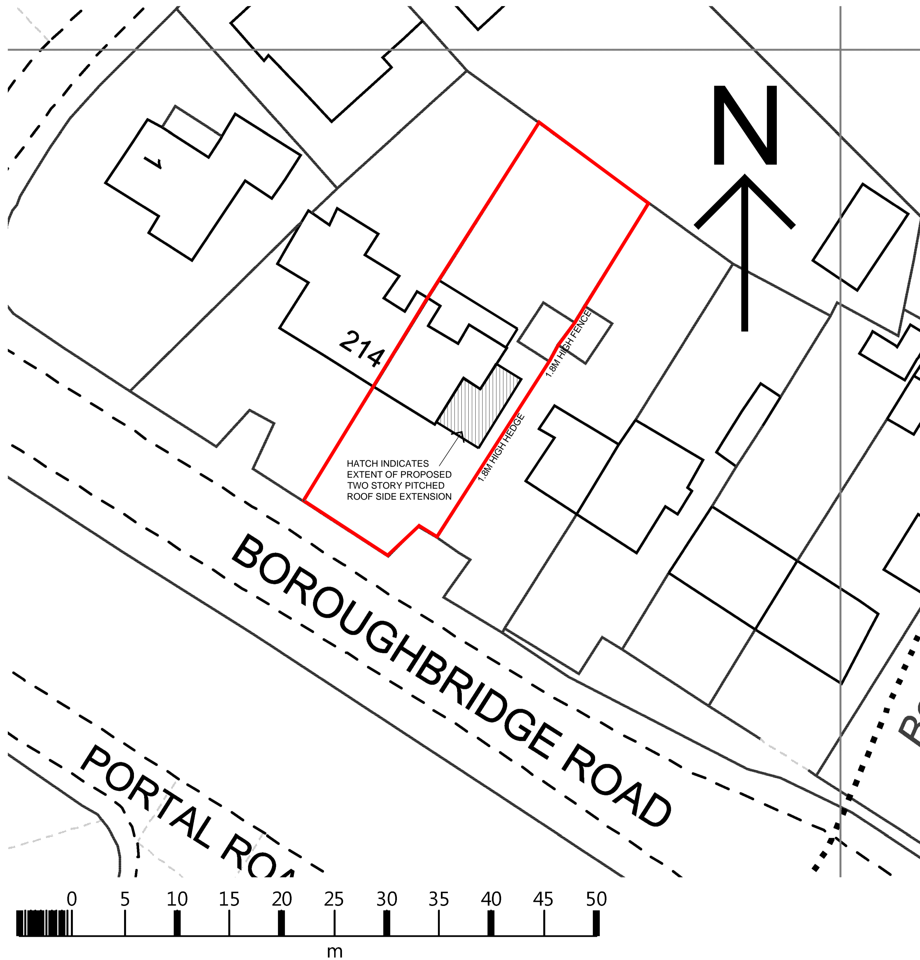
BLOCK PLAN
