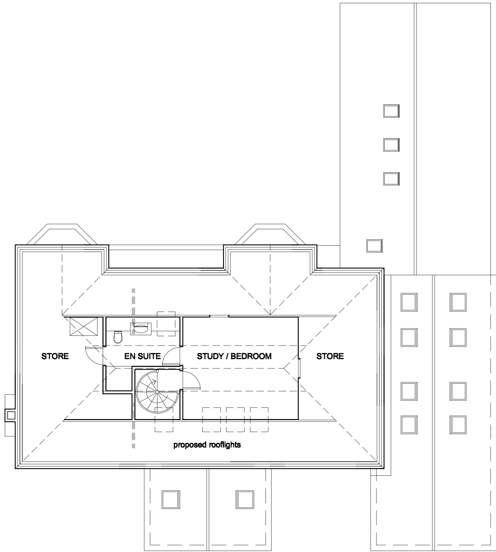
ROOF PLAN
