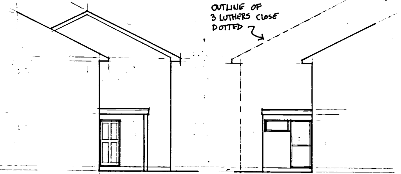
EXISTING SIDE ELEVATIONS 1:100
