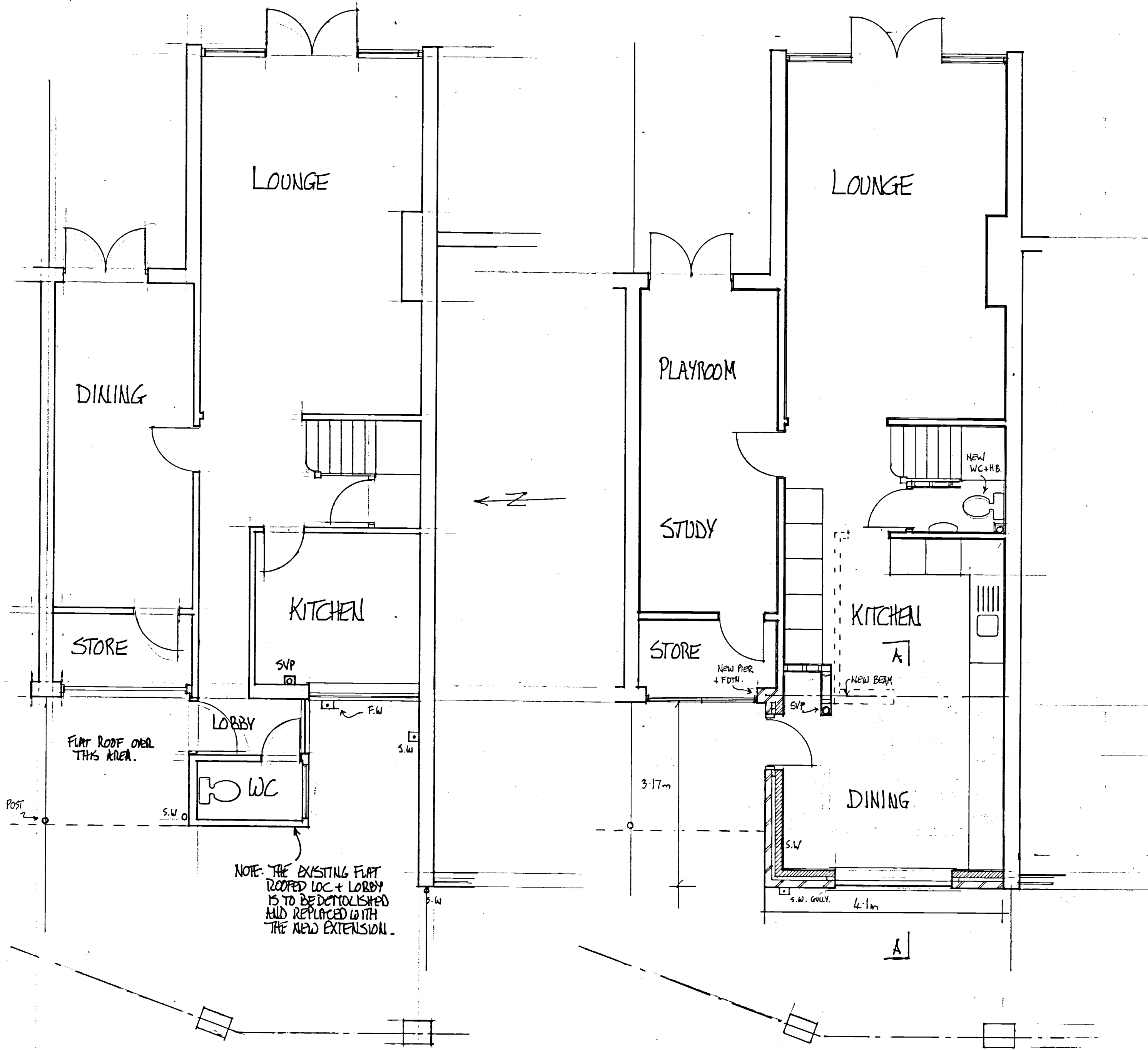
PROPOSED GROUND FLOOR 1:50
