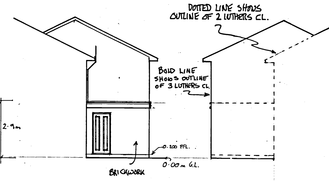
PROPOSED SIDE ELEVATIONS 1:100
