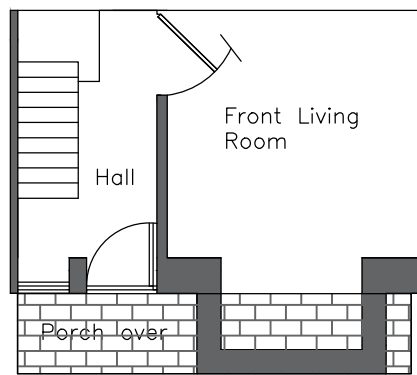
Floor Plan 1:100
