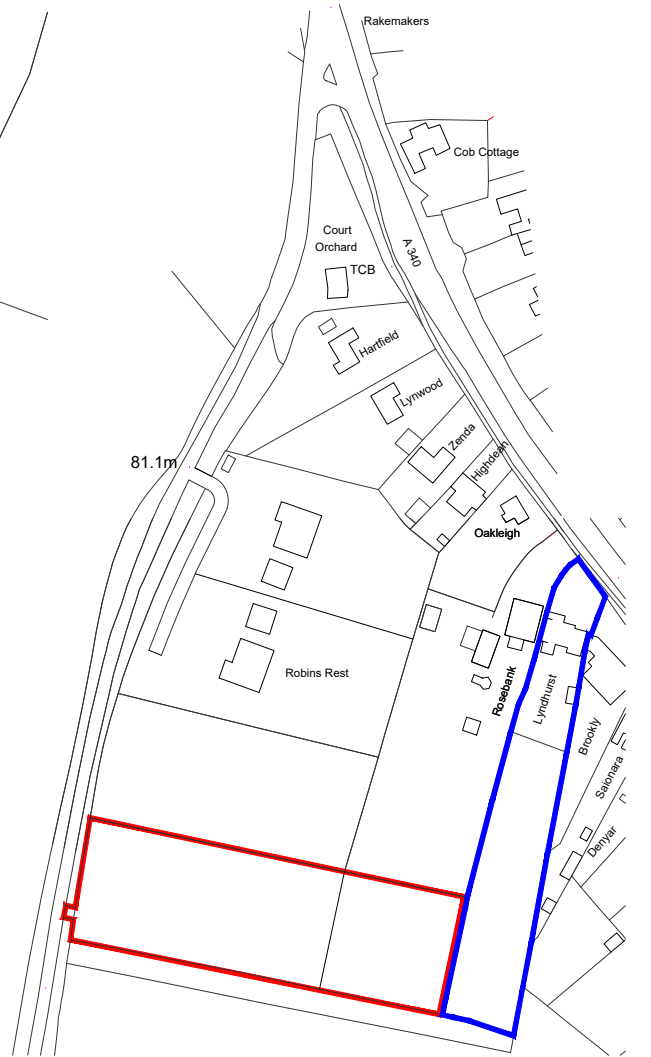
LOCATION PLAN Scale 1:2500 Site Area = 4985sqm
