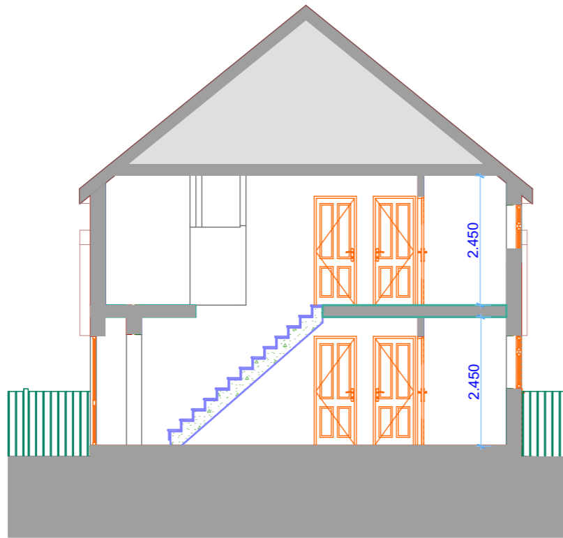
S-01 Building Section 1:100
