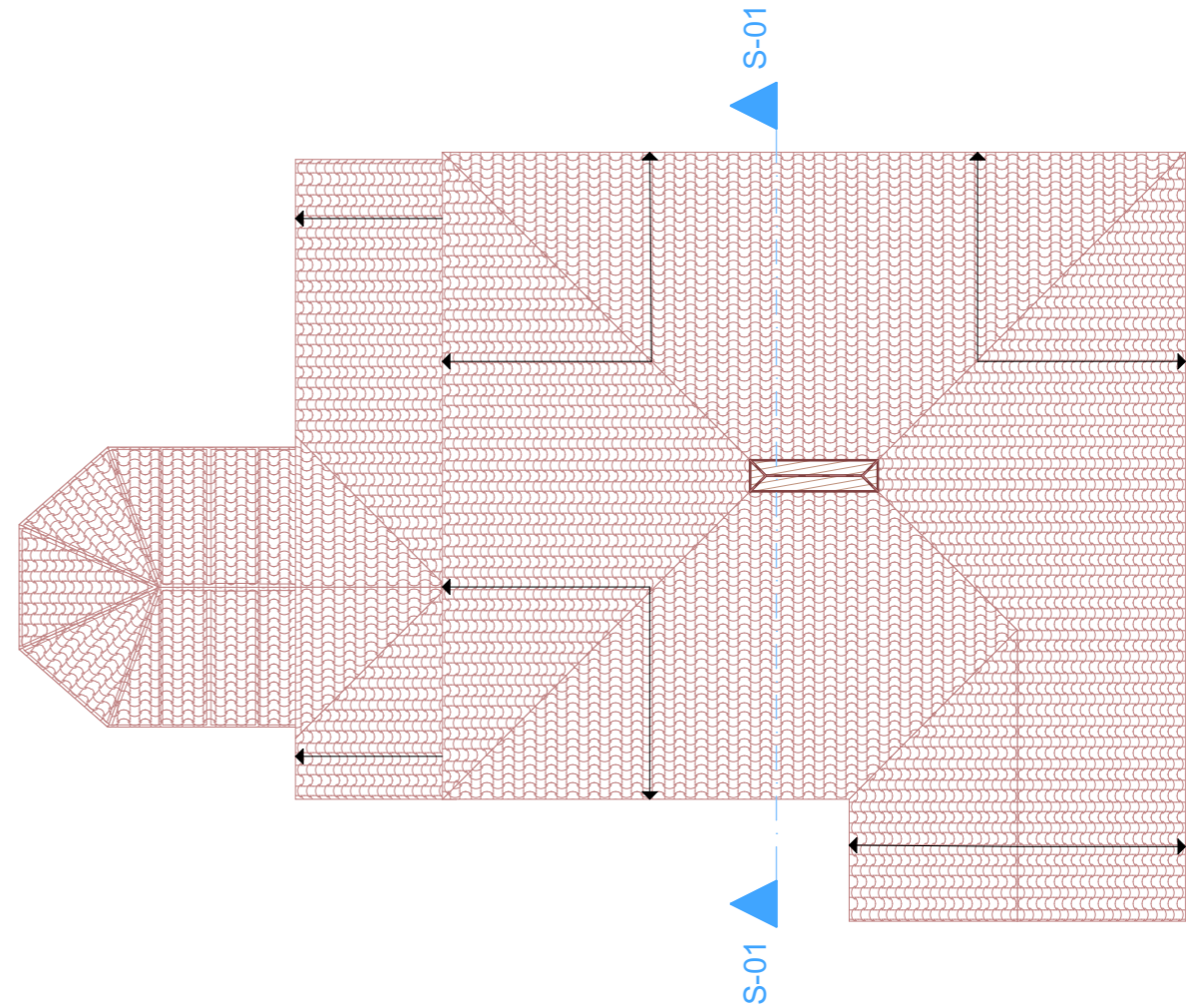
Roof Plan 1:100
