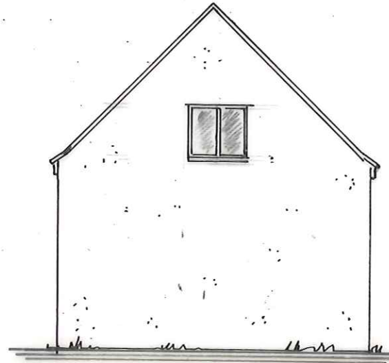
SIDE EL.
