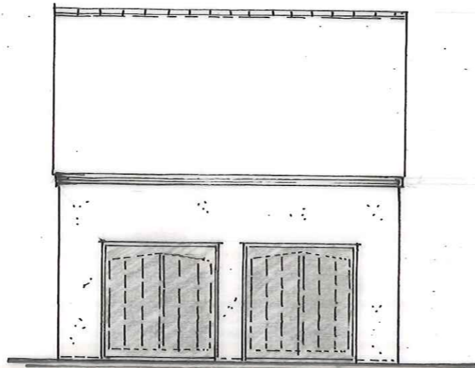
FRONT EL.
