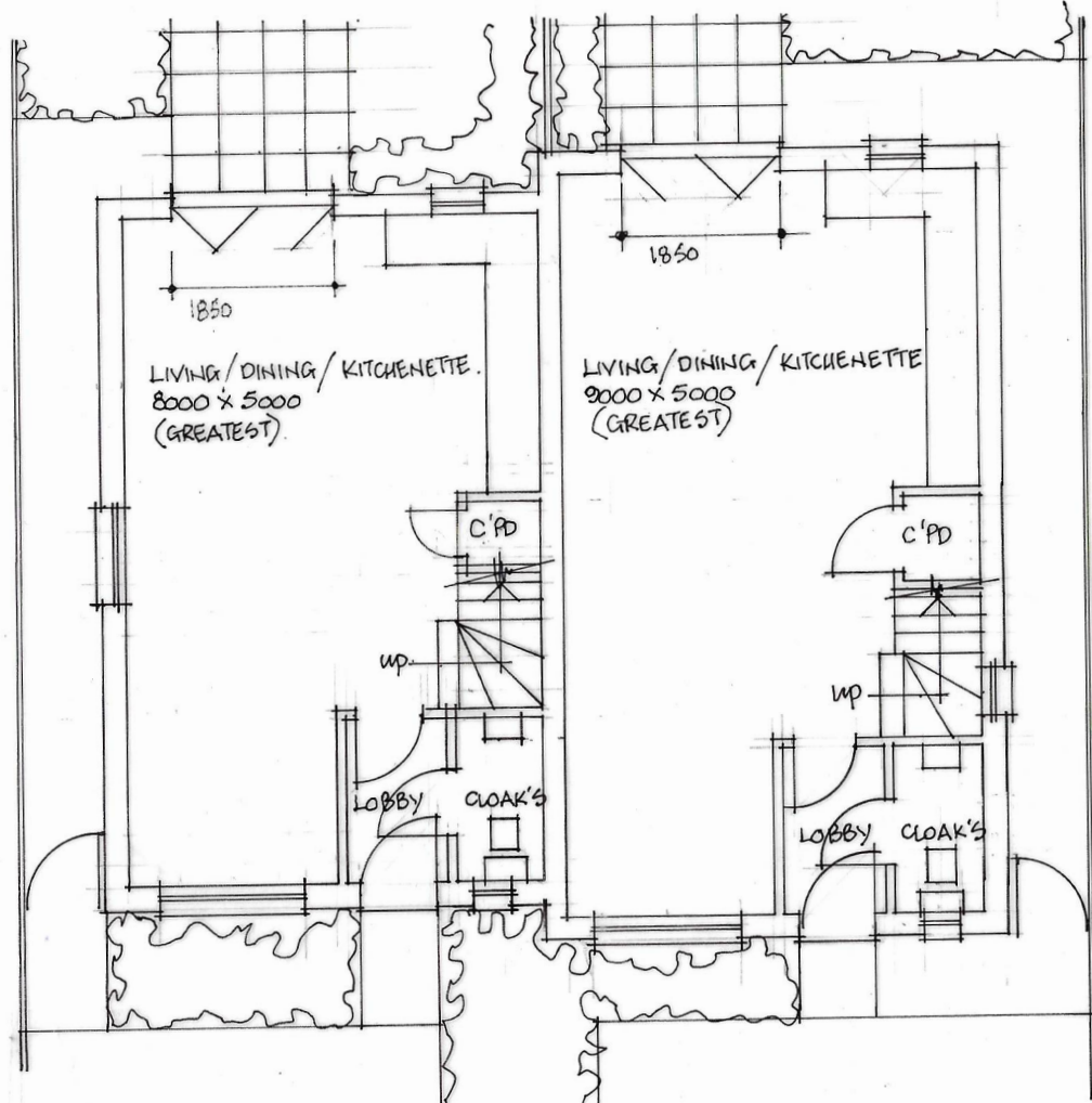
GROUND FLOOR PLAN TYPE A
