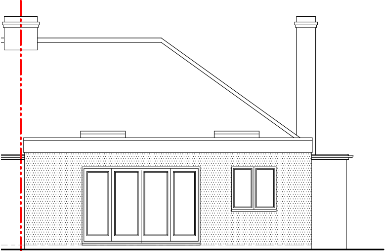
REAR ELEVATION AS PROPOSED
