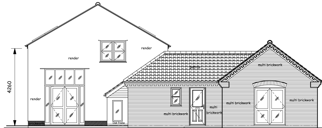
EAST ELEVATION
