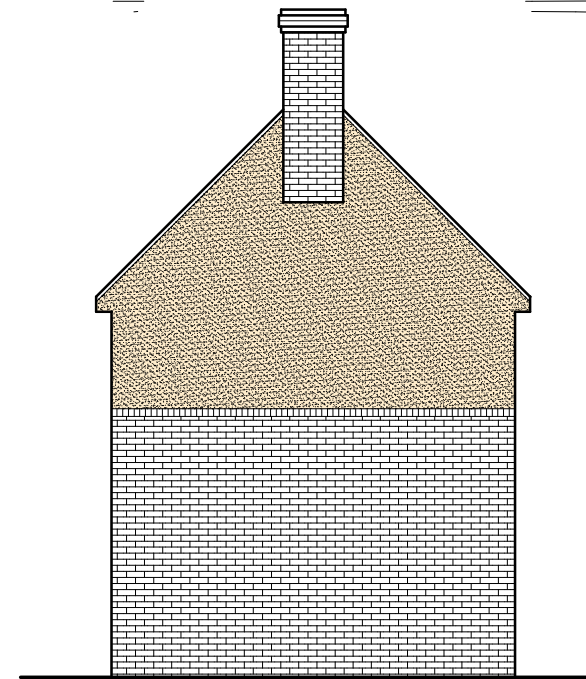
Side Elevation as Existing.
