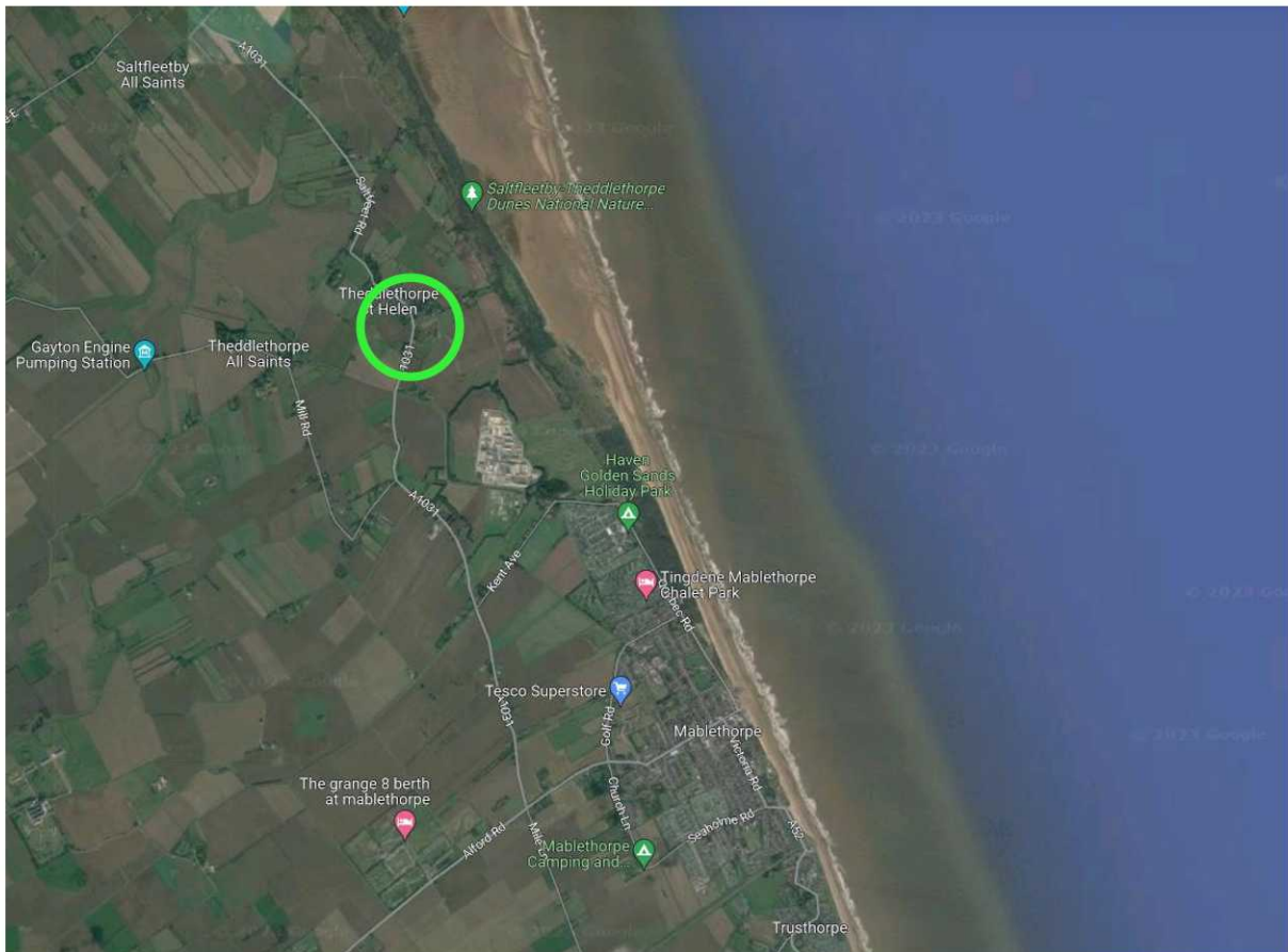
Figure 2: Aerial photograph showing the location of the site in relation to Skegness.
