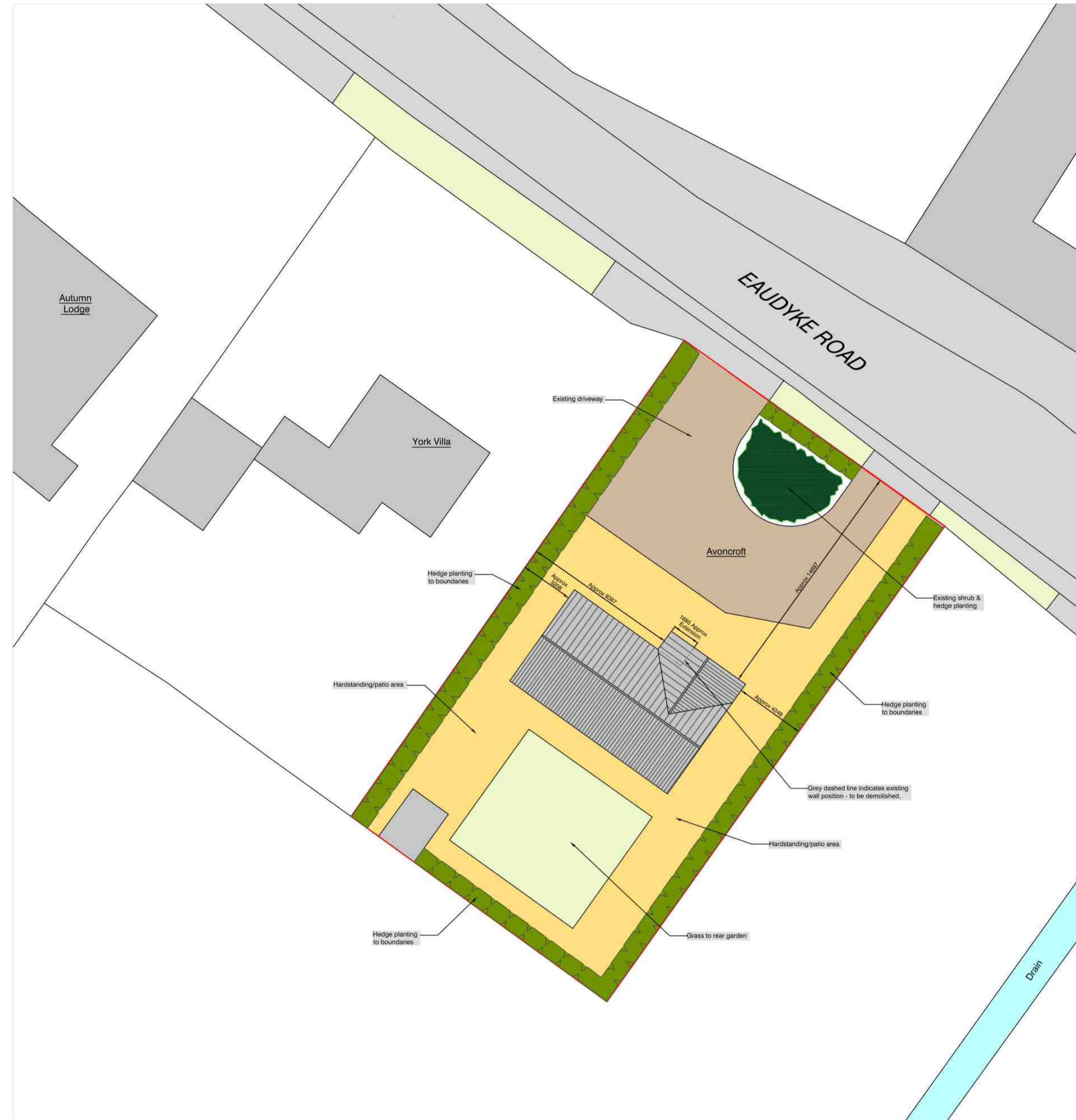
Proposed Block Plan 1:200 @ A1
