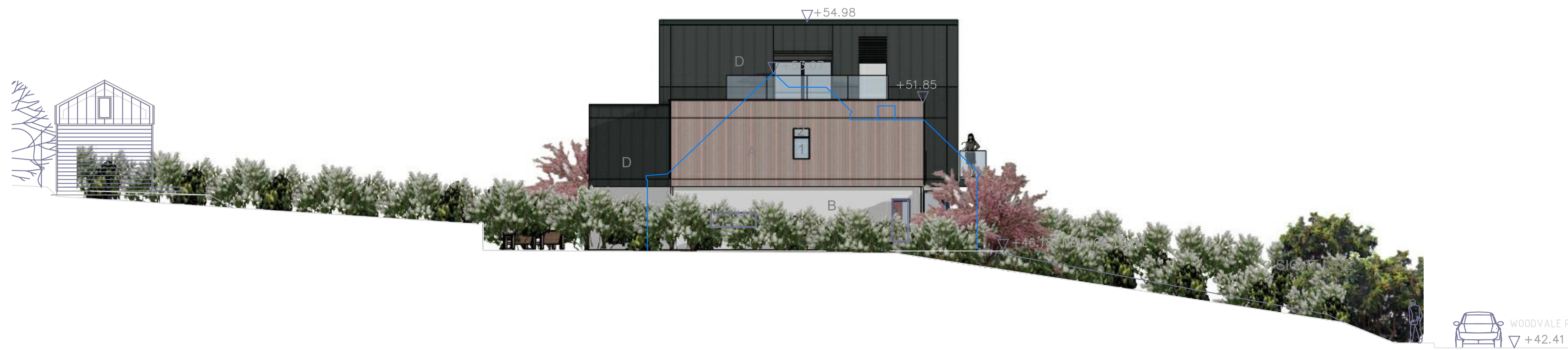
NORTH ELEVATION -1:100 scale @ A1 existing house outline
