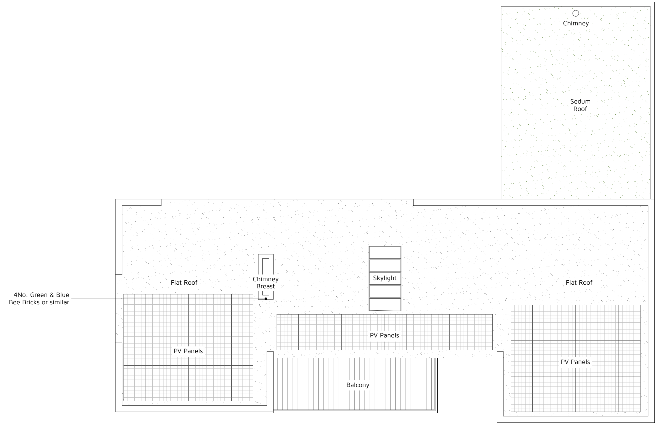
Proposed Roof Plan 1:100 @ A3
