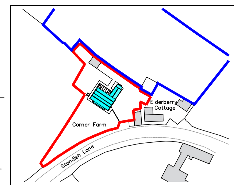
LOCATION PLAN 1:1250
