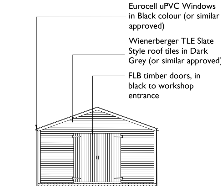
04 Side Elevation - As Proposed 203 1:100
