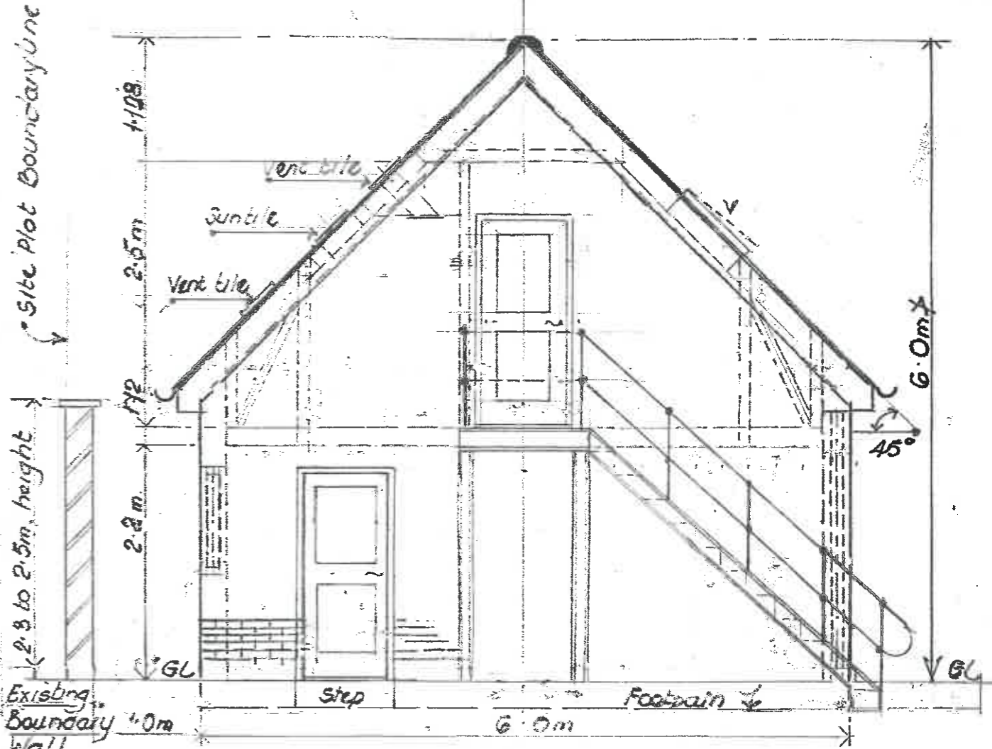
Side View (South Elevation) View from Inside Garden
