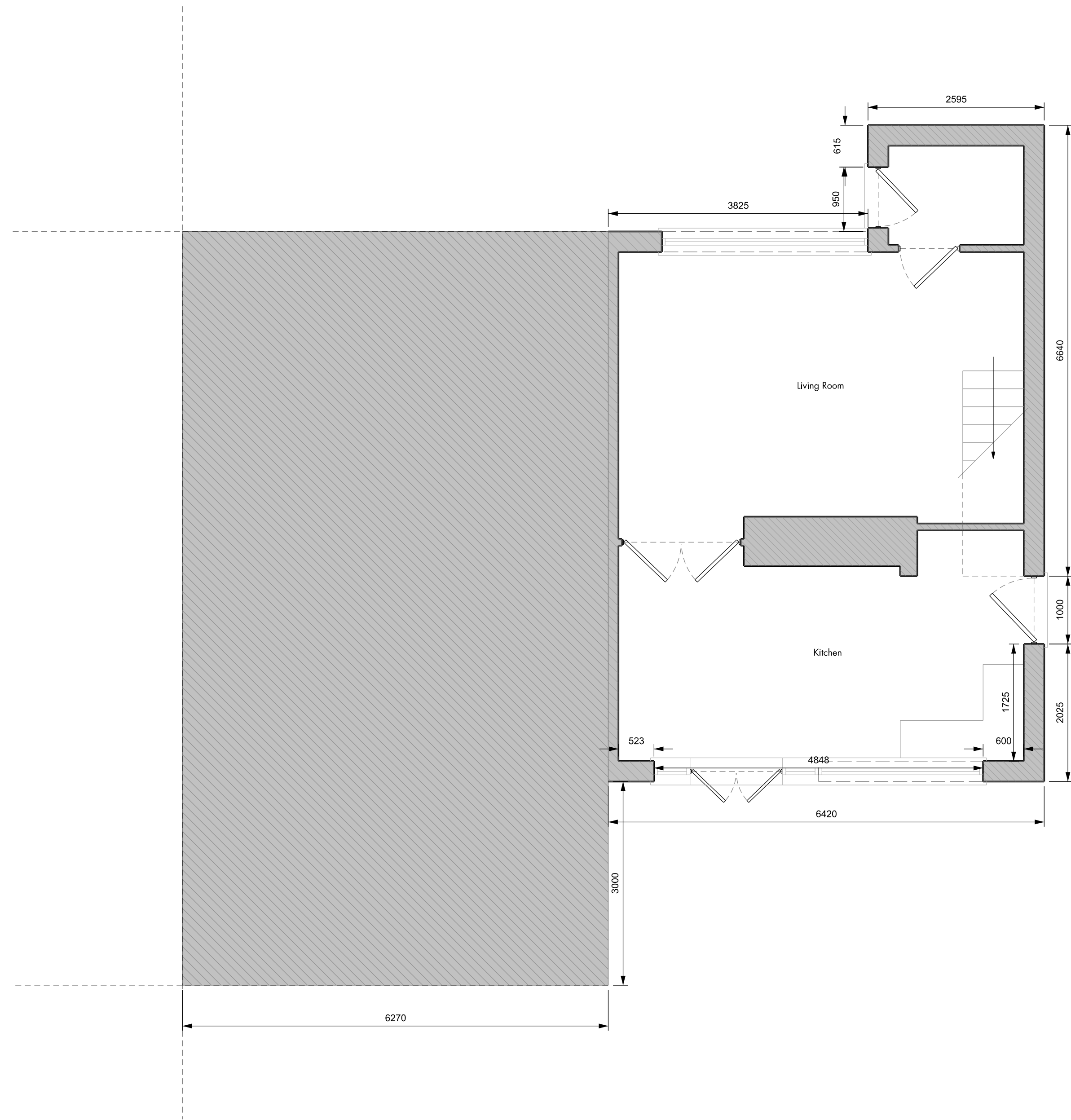
Existing Ground Floor Plan 1:50
