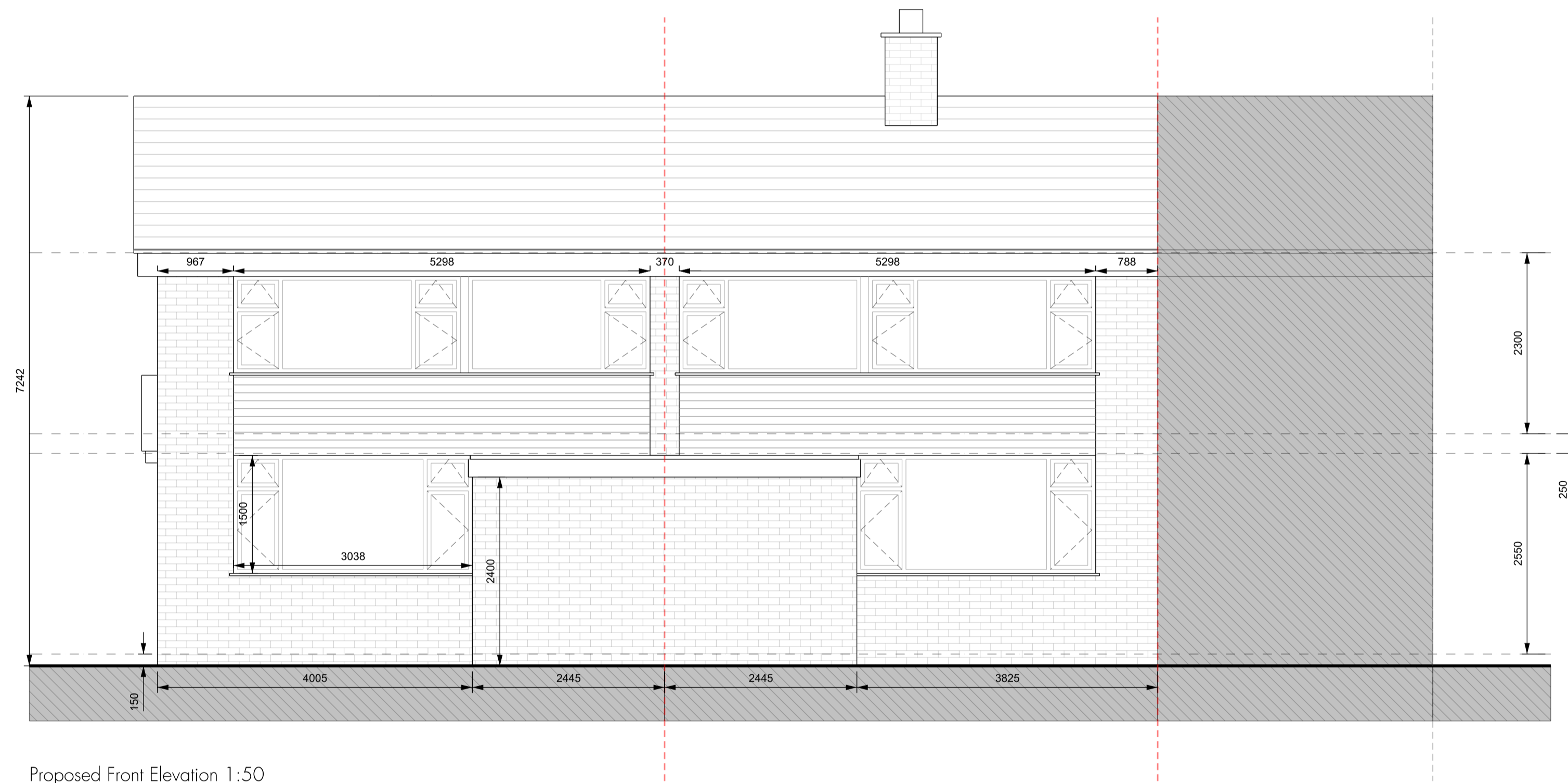
Proposed Front Elevation 1:50
