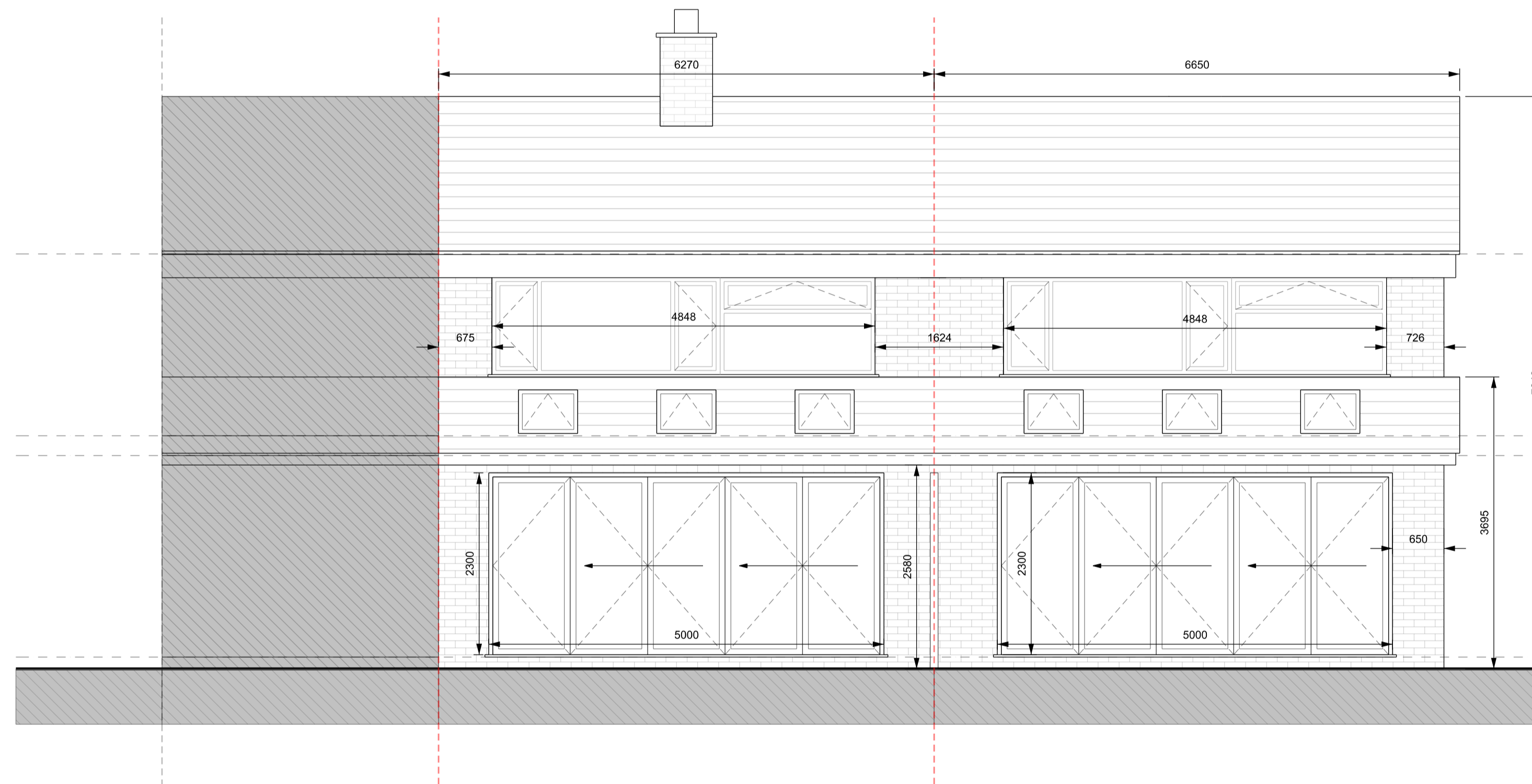
Proposed Rear Elevation 1:50
