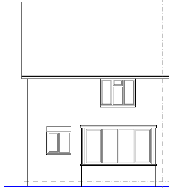
REAR ELEVATION
