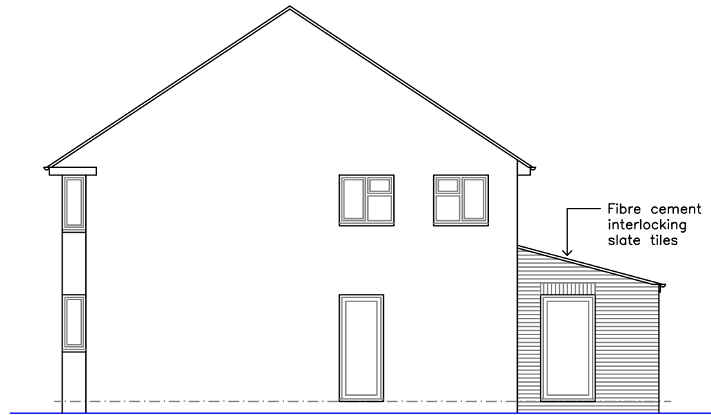
SIDE ELEVATION
