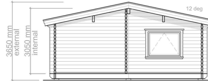
South Elevation
