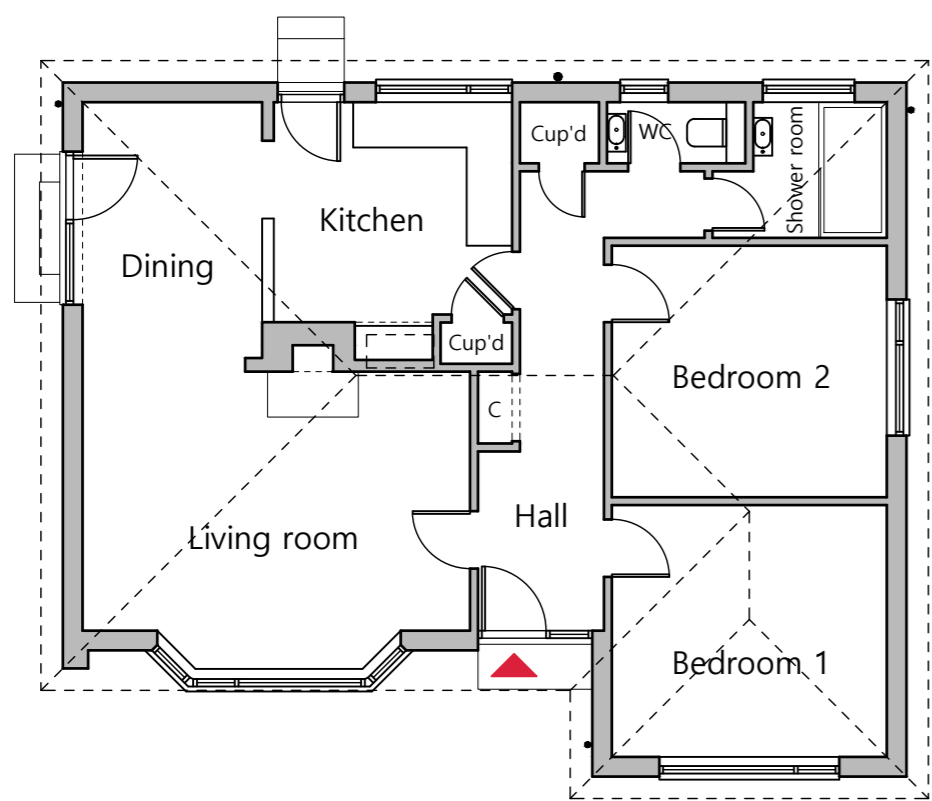
Existing floor plan 1:100 (Roof plan shown dashed)
