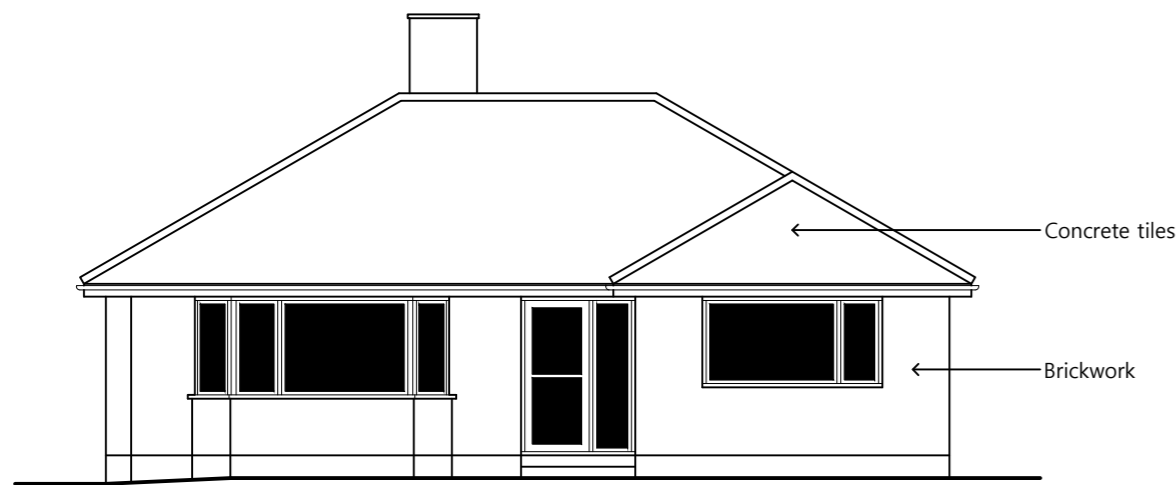
Existing front (east) elevation 1:100
