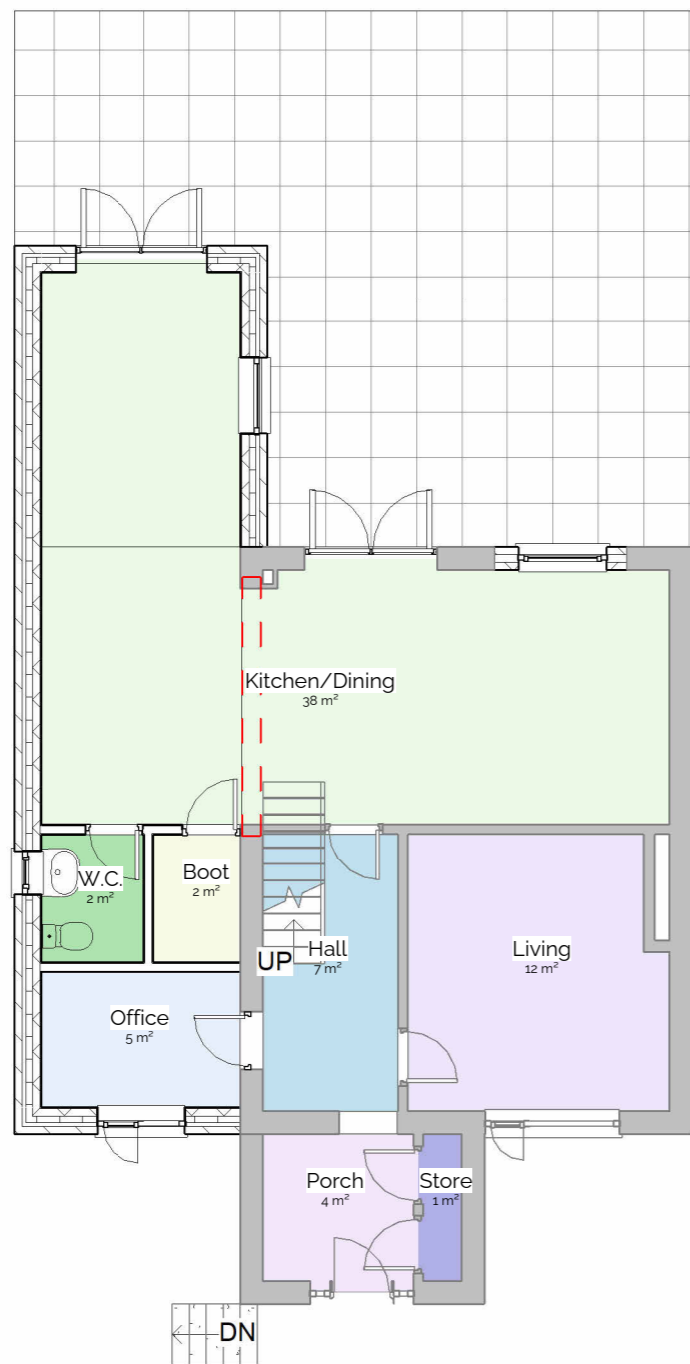
1 Ground 1 : 100
