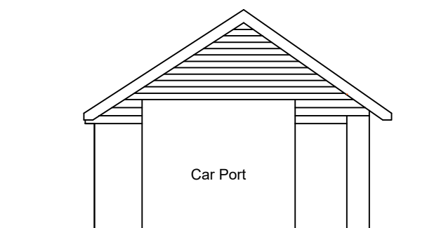
East Elevation 1:100
