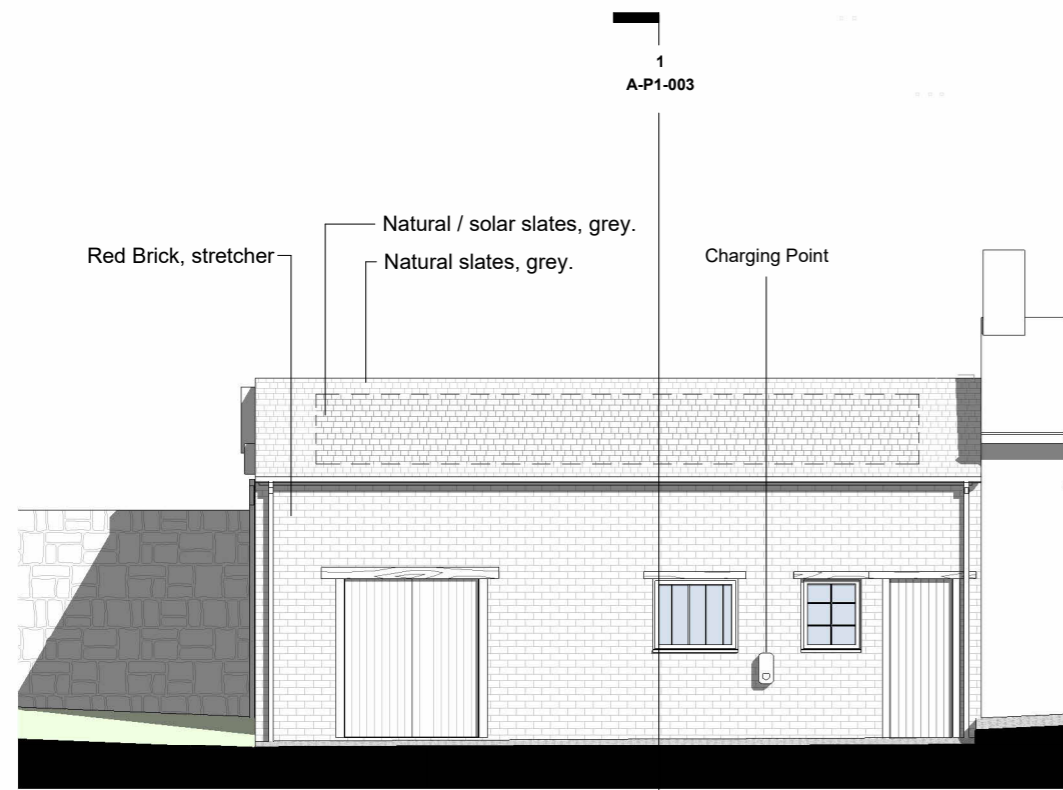
Proposed Elevation 03
