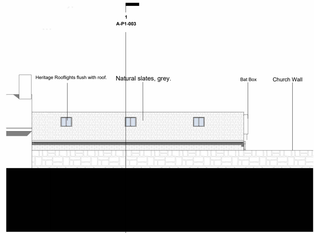
Proposed Elevation 02
