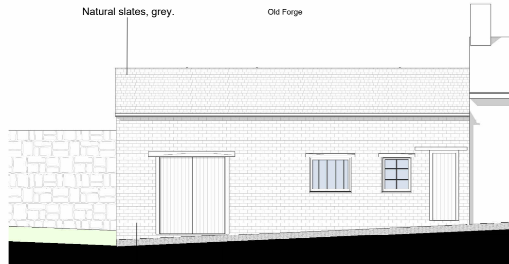
Existing Elevation 03
