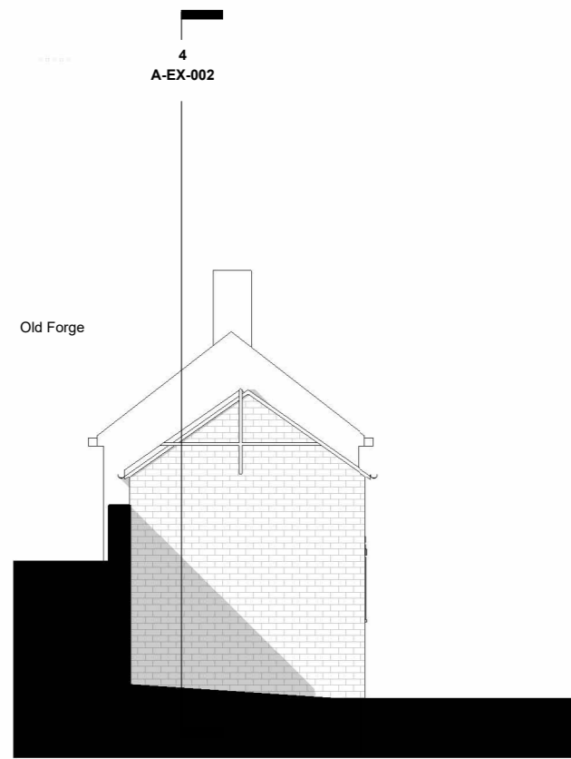
Existing Elevation 01
