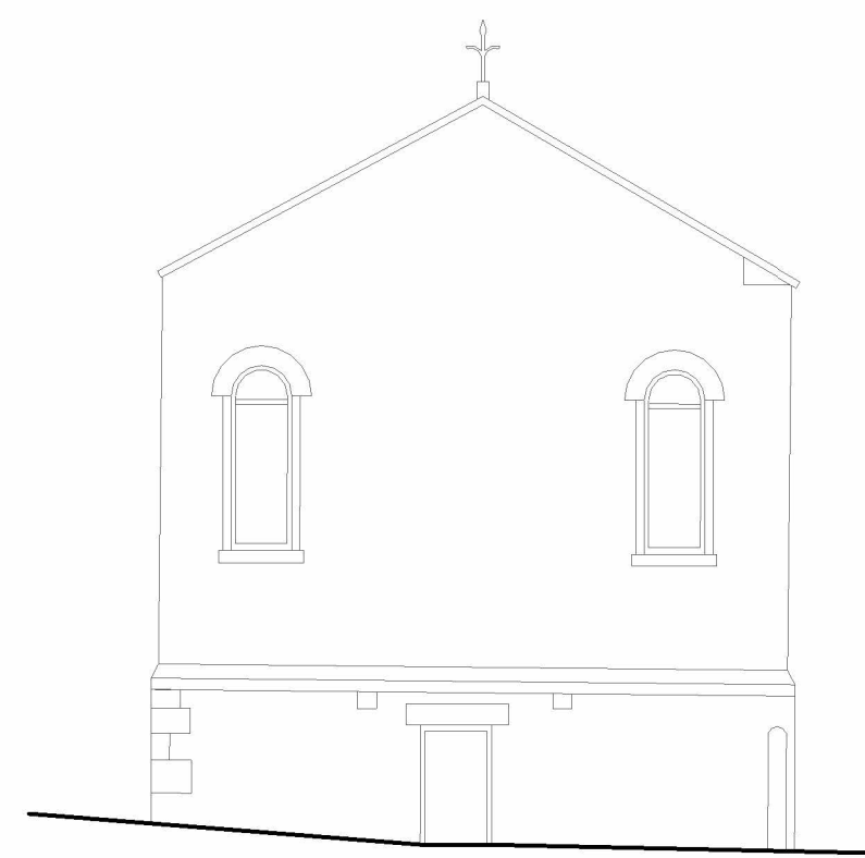
3 North Elevation - Existing - Survey 1 : 100
