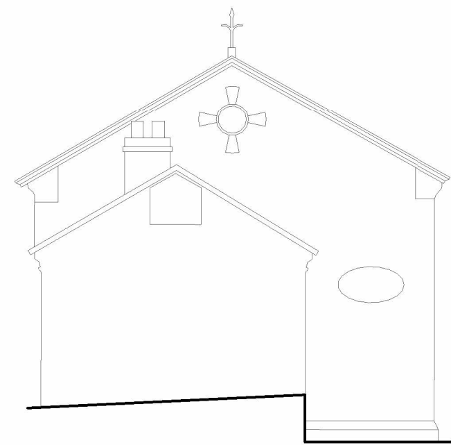
3 North Elevation - Existing - Survey 1 : 100
