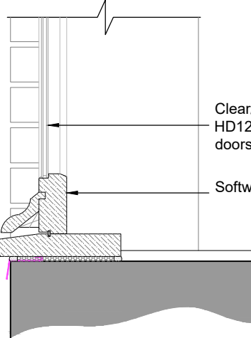
CASEMENT FRENCH DOORS DG01 ELEVATIONAL SECTION
