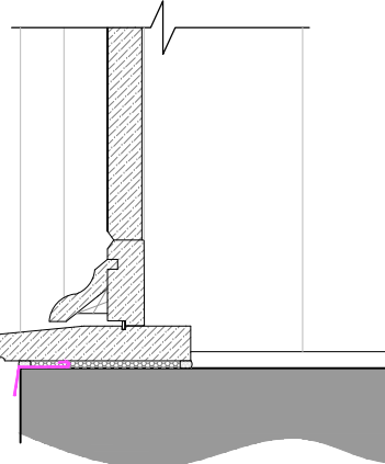
CASEMENT DOOR DG02 ELEVATIONAL SECTION
