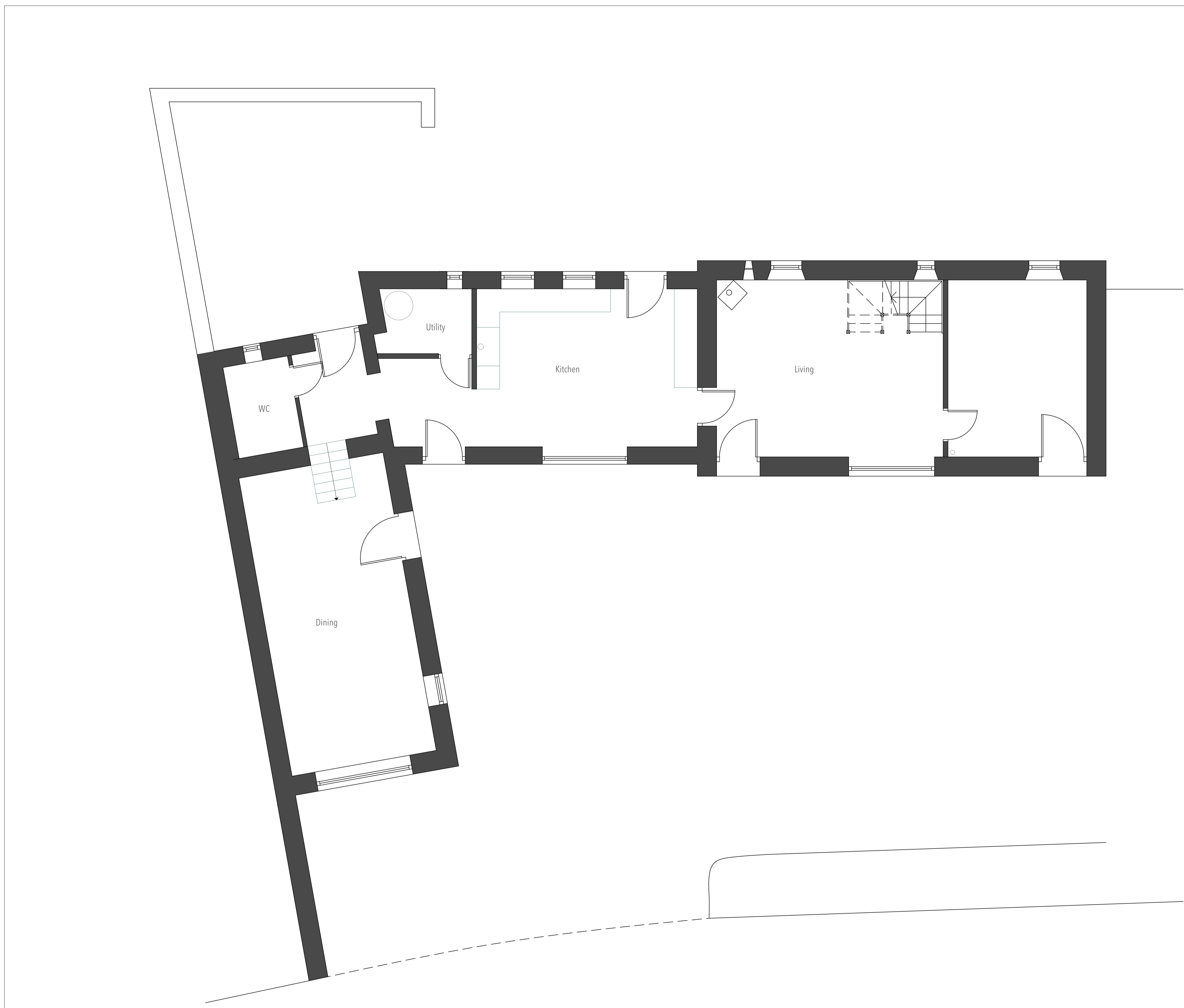
Proposed Ground Floor Plan 1:50
