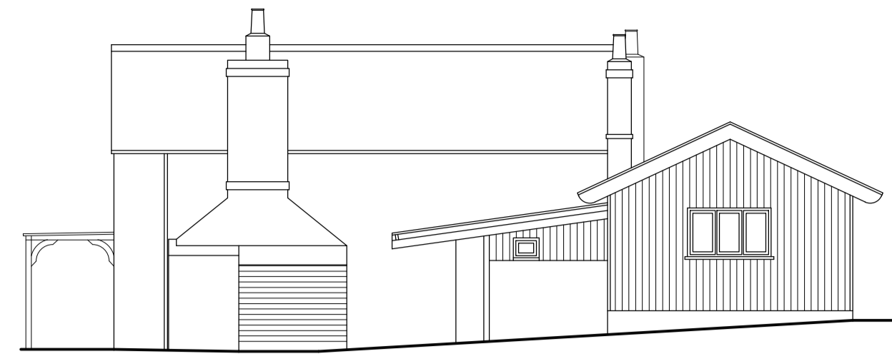
Side Elevation
