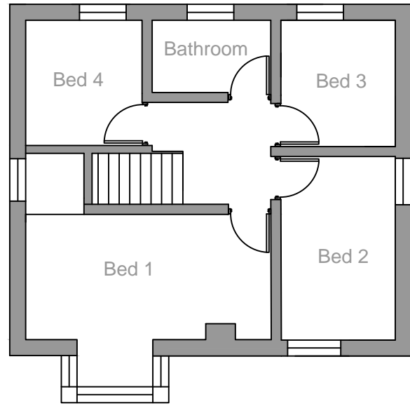
Existing first floor
