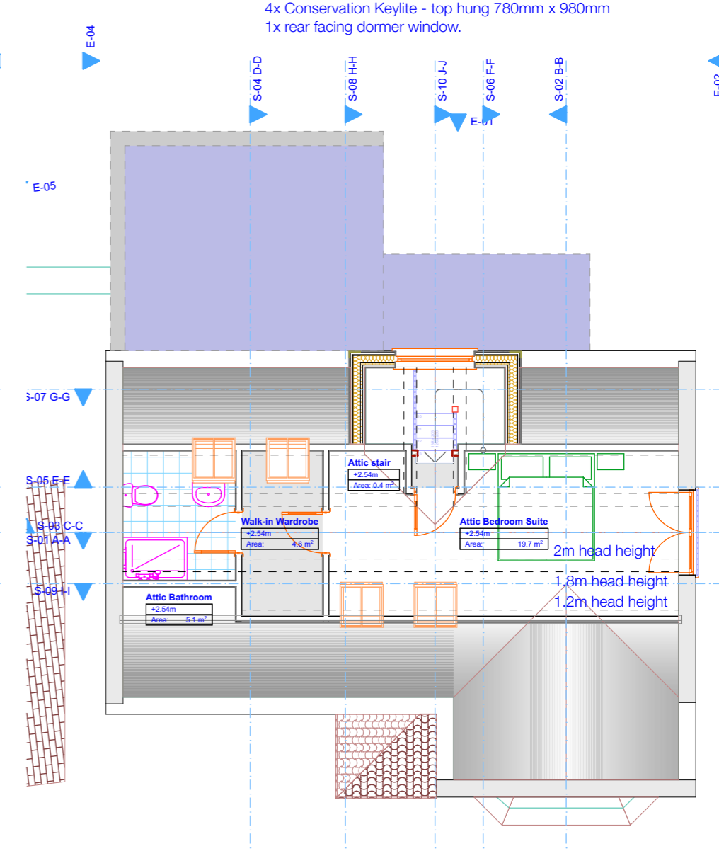
2. 02-Attic Floor Proposed 1:100
