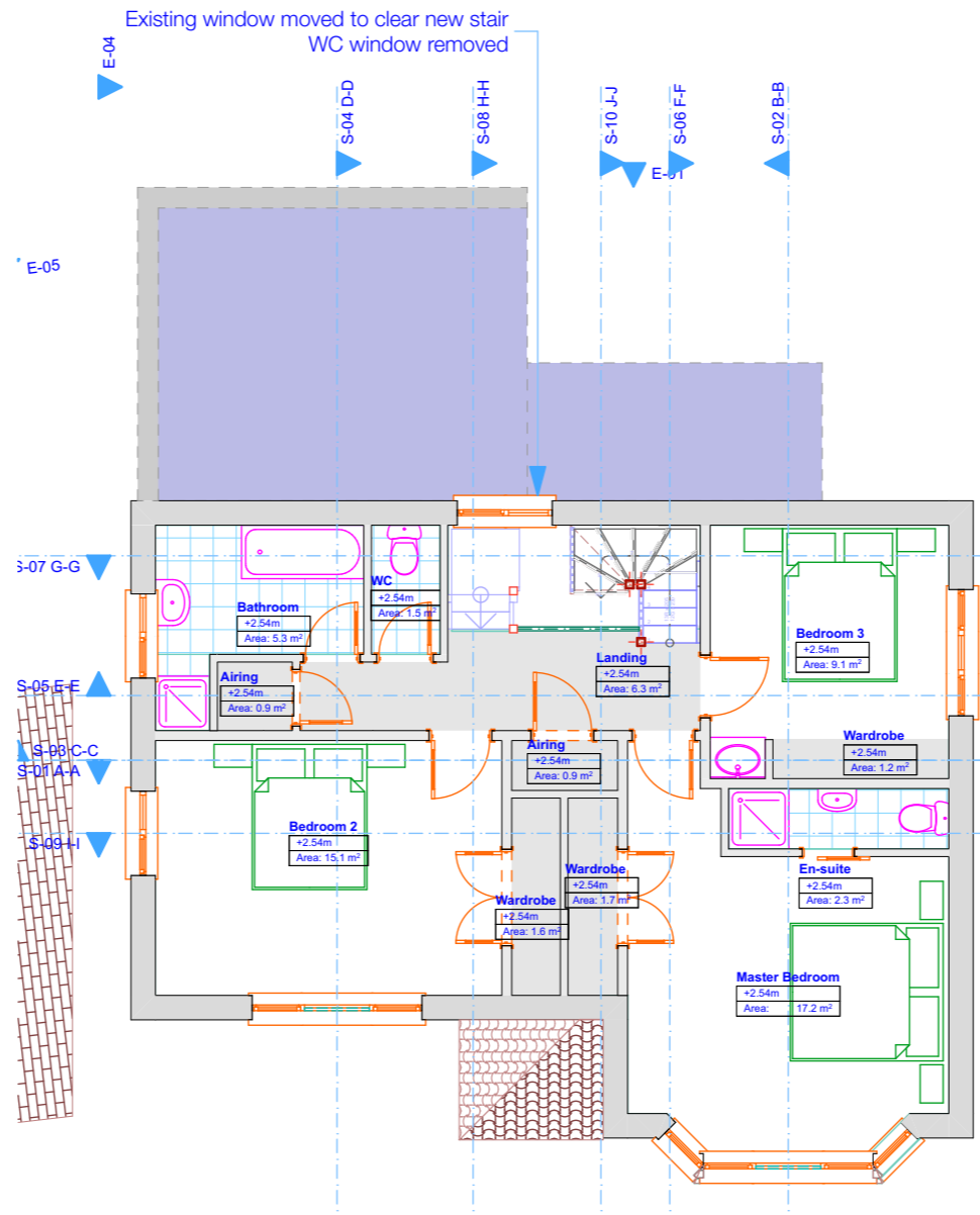
1. 01-First Floor Proposed 1:100
