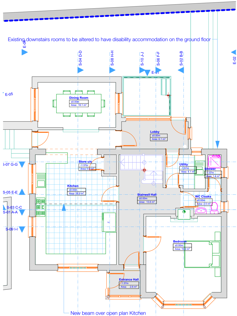
0. 00-Ground Floor Proposed 1:100
