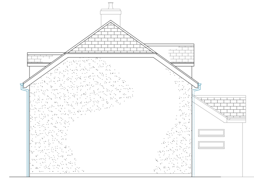
West scale 1:100
