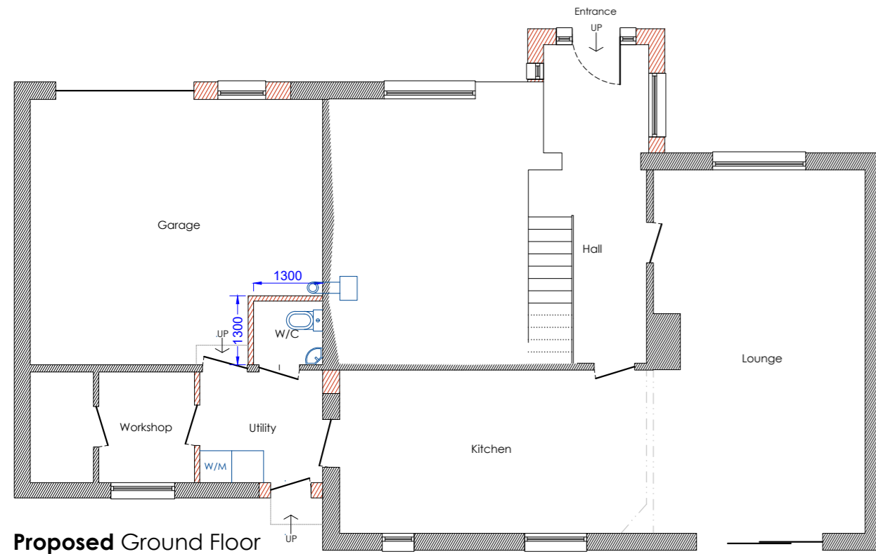
Proposed Ground Floor scale 1:100
