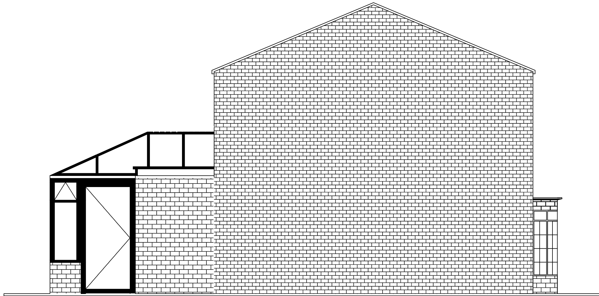
West elevation proposed
