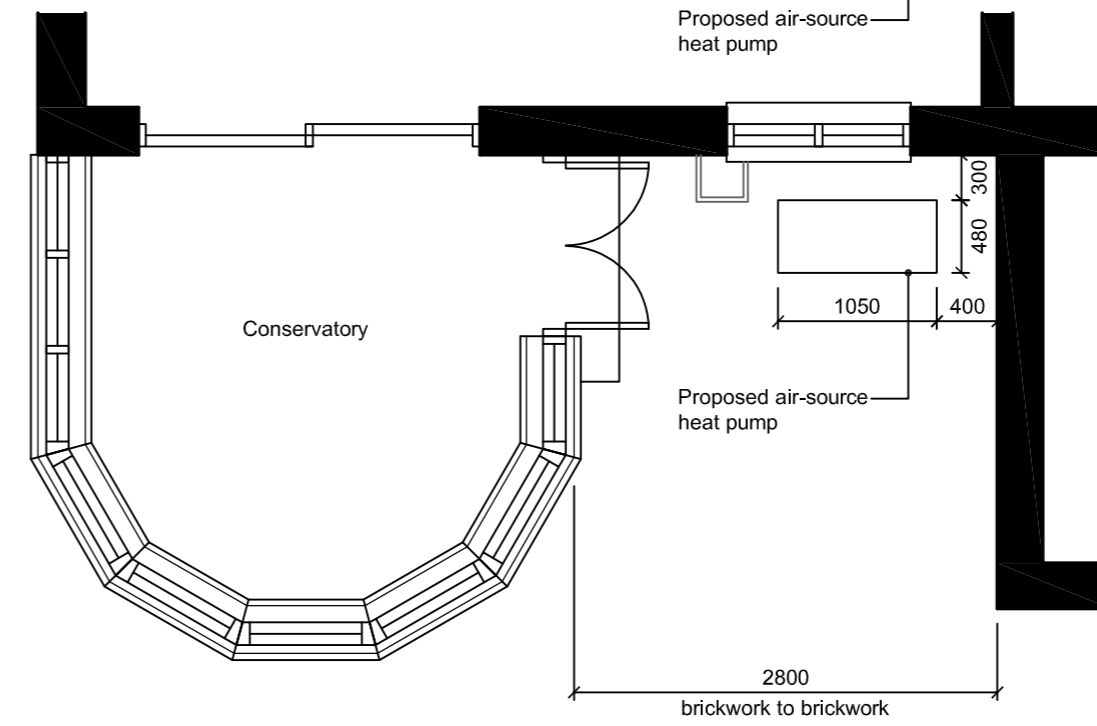
Plan & Elevation as Proposed
