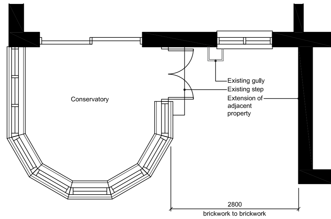
Plan & Elevation as Existing
