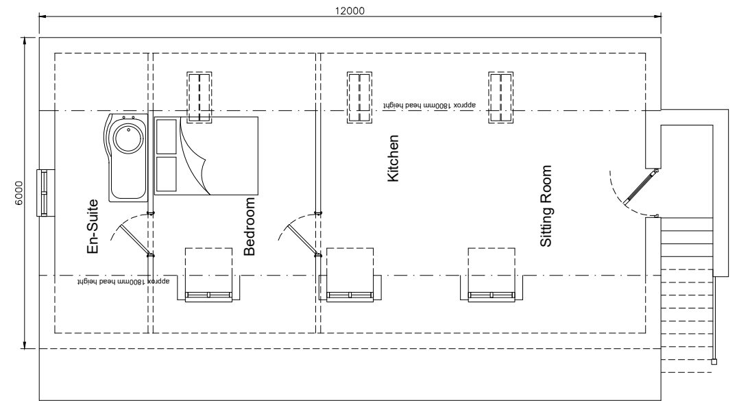
Annexe First Floor
