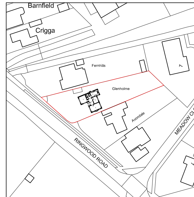
Location Plan (1:1250)
