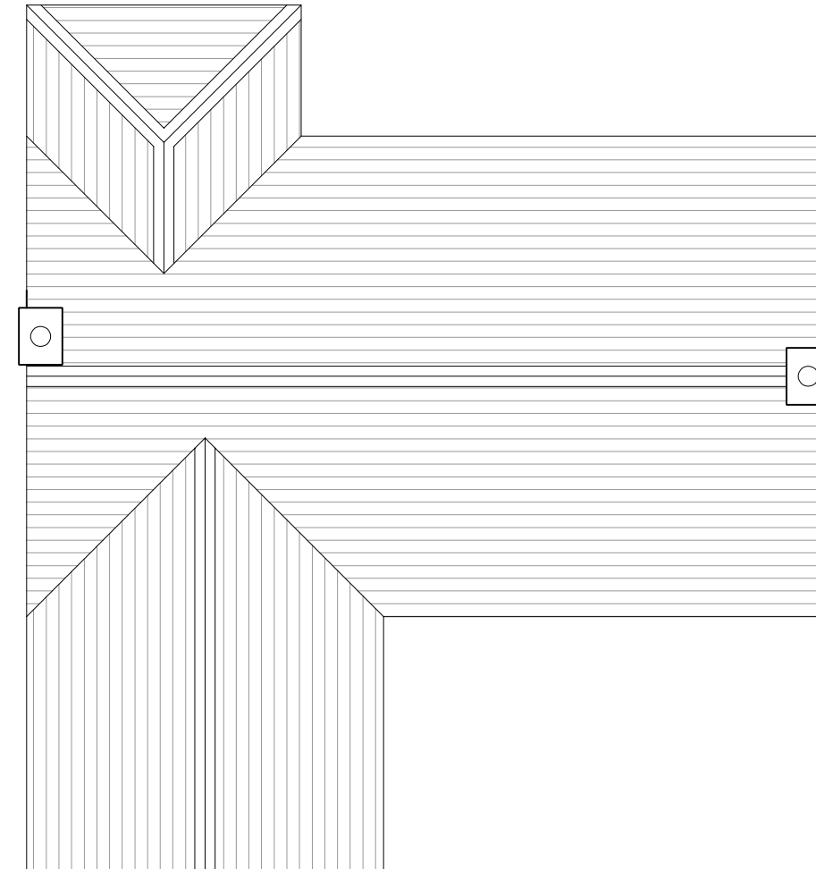
Roof Plan 1:100
