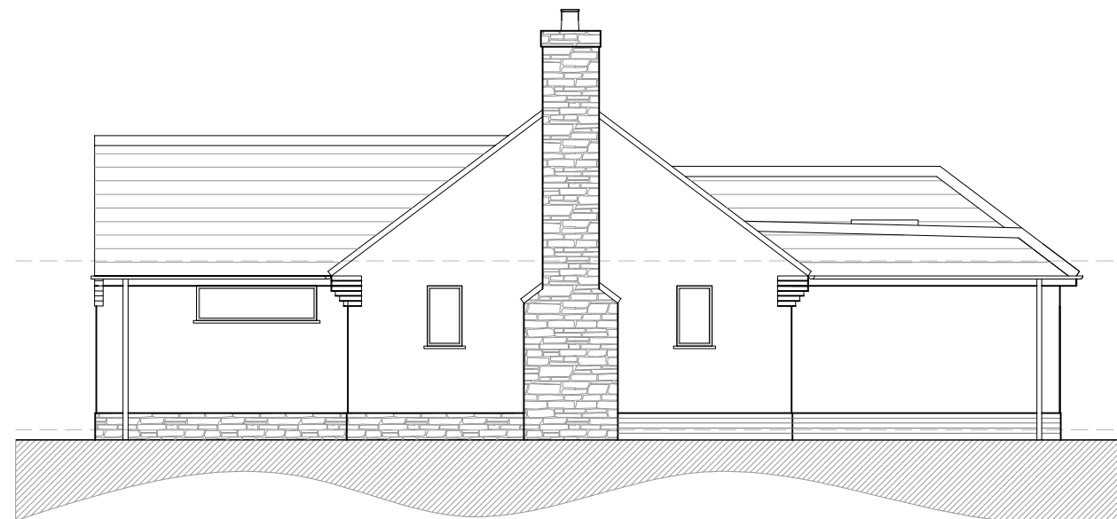
Side (South East) Elevation
